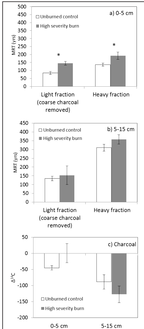
Figure 2. Modeled mean residence times (MRT) of density fractions from high-severity burn and unburned control soils at two depths: a) 0 cm to 5 cm, and b) 5 cm to 15 cm. c) \Delta^{14}\text{C} (‰) of coarse charcoal removed from the 0 cm to 5 cm and 5 cm to 15 cm depths of high-severity burn and unburned soils. Error bars are the standard error of either 5 or 6 experimental replicates. Asterisks (*) indicate significant differences between control and burnt soils at \alpha = 0.05 .
